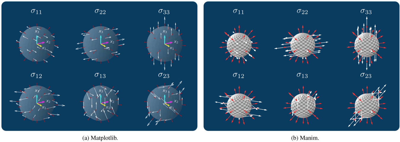
FIGURE 2 | Animation of the six independent stress components in a fixed Cartesian basis. Outward unit normal vectors (red) and traction vectors (white) are shown at selected points on infinitesimal volume elements. For the animated version of (a), see https://github.com/DrSimulate/gallery .
