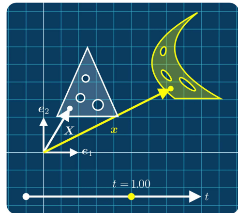
FIGURE 3 | Animation of nonlinear kinematics in continuum mechanics. A two-dimensional example is considered for simplicity. For the animated version, see https://github.com/DrSimulate/gallery .
