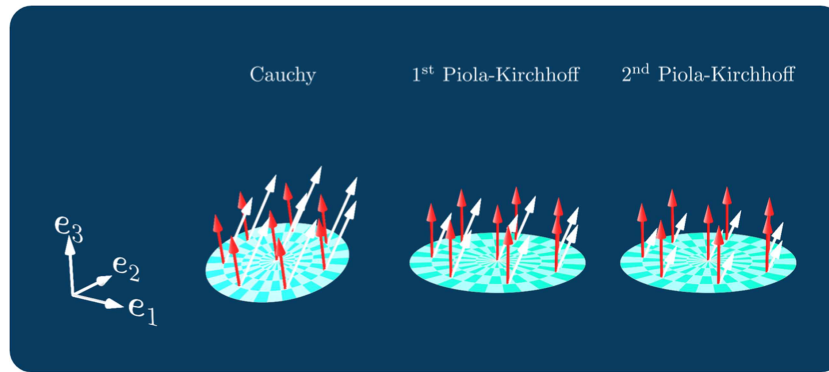
FIGURE 9 | Illustration of undeformed and deformed area elements with surface normals (red) and tractions (white) corresponding to the Cauchy stress (left), the first Piola-Kirchhoff stress (center), and the second Piola-Kirchhoff stress (right). Animating the rotation of the area elements highlights that stress tensors encode the tractions acting on arbitrarily oriented surfaces. For the animated version, see https://github.com/DrSimulate/gallery .
