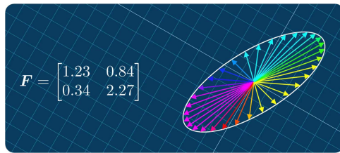
FIGURE 6 | Animation of the effect of the deformation gradient tensor on a set of undeformed line element vectors on the unit circle in a Cartesian basis. A two-dimensional example is considered for simplicity. For the animated version, see https://github.com/DrSimulate/gallery .
