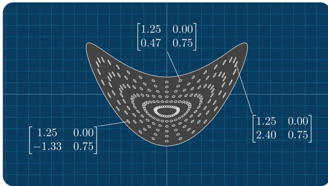
FIGURE 7 | Animation of nonlinear kinematics in continuum mechanics. The deformation gradient tensor field is visualized by animating the deformation of infinitesimal volume elements (or area elements in the two-dimensional case) at selected points. A two-dimensional example is considered for simplicity. For the animated version, see https://github.com/DrSimulate/gallery .
