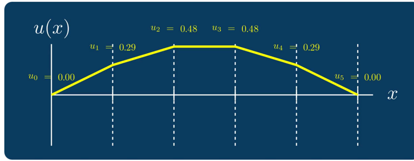
FIGURE 10 | Animation of a parameterized solution function in finite element analysis. A one-dimensional example is considered for simplicity. For the animated version, see https://github.com/DrSimulate/gallery .
