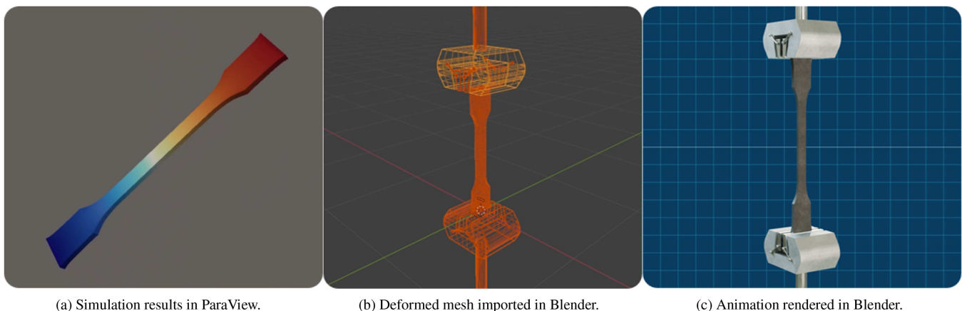
FIGURE 4 | Animation of finite element simulation results in Blender. For the animated version, see https://github.com/DrSimulate/gallery .
