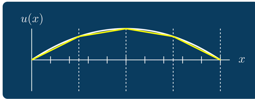
FIGURE 11 | Animation of mesh refinement in finite element analysis. The analytical solution is shown in white, and the finite element solution is shown in yellow. A one-dimensional example is considered for simplicity. For the animated version, see https://github.com/DrSimulate/gallery .
