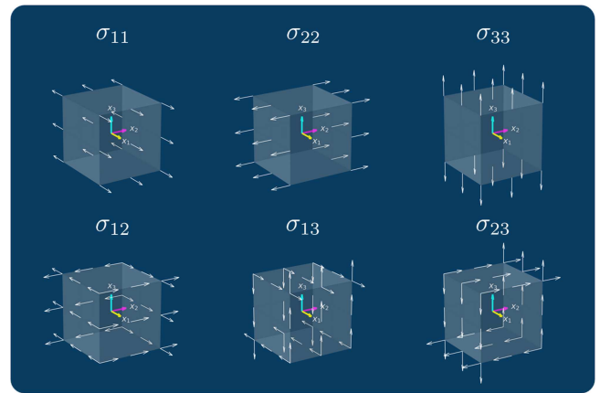
FIGURE 8 | Animation of the six independent stress components in a fixed Cartesian basis. Traction vectors are shown at selected points on infinitesimal volume elements. For the animated version, see https://github.com/DrSimulate/gallery .
